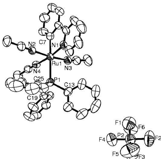
Figure 1. ORTEP view of compound 7 . Selected bond distances [Å] and angles [°]: Ru1–N2 2.009(3), Ru1–N(4) 2.026(3), Ru1–N3 2.039(3), Ru1–C7 2.049(4), Ru1–N1 2.088(3), Ru1–P1 2.458(1); N2–Ru1–N4 87.89(11), N2–Ru1–N3 172.84(11), N4–Ru1–N3 91.65(11), N2–Ru1–C7 87.63(12), N4–Ru1–C7 92.85(13), N3–Ru1–C7 85.26(12), N2–Ru1–N1 87.46(10), N4–Ru1–N1 171.53(11).
