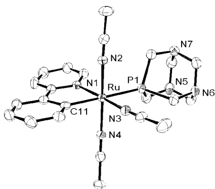
Figure 2. ORTEP view of the cation of 8 . Selected bond distances [Å] and angles [°]: Ru1–N2 2.013(2), Ru1–N4 2.022(2), Ru1–N3 2.024(2), Ru1–C11 2.068(3), Ru1–N1 2.087(2), Ru1–P1 2.395(1); N2–Ru1–N4 175.34(8), N2–Ru1–N3 88.70(8), N4–Ru1–N3 87.91(7), N2–Ru1–C11 90.75(8), N4–Ru1–C11 90.75(8), N3–Ru1–C11 95.46(9), N2–Ru1–N1 89.66(7), N4–Ru1–N1 93.41(7).
