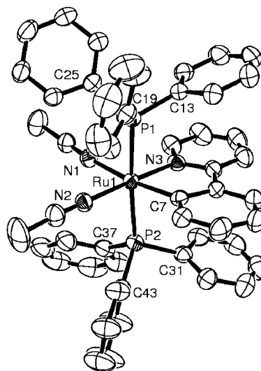
Figure 3. ORTEP view of the cationic part of compound 9 . Selected bond distances [Å] and angles [°]: Ru1–N2 2.026(3), Ru1–N3 2.065(3), Ru1–C7 2.058(4), Ru1–N1 2.134(3), Ru1–P1 2.3765(9), Ru1–P2 2.3781(9); N2–Ru1–P1 92.94(8), N2–Ru1–N3 177.20(10), P2–Ru1–N3 88.73(7), N2–Ru1–C7 101.57(12), N1–Ru1–C7 171.72(11), N3–Ru1–C7 79.22(12), N2–Ru1–N1 86.19(10).
