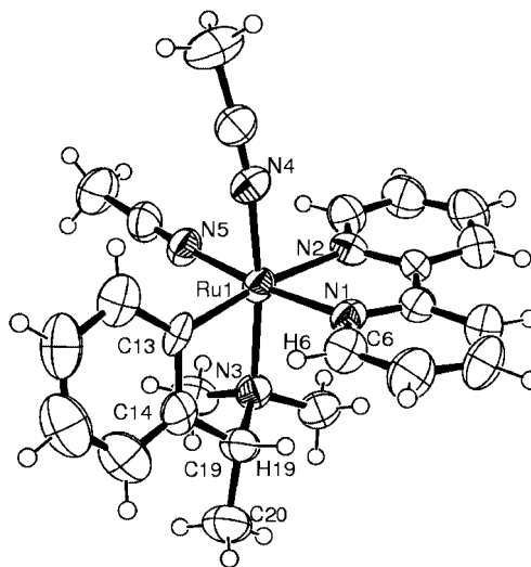
Figure 5. ORTEP view of the cationic part of compound 18 . Selected bond distances [Å] and angles [°]: Ru1–N3 2.175(5), Ru1–N4 2.018(5), Ru1–N5 2.001(5), Ru1–C13 2.027(6), Ru1–N1 2.057(5), Ru1–N2 2.148(5); N2–Ru1–N1 78.16(19), N2–Ru1–N3 96.69(18), N3–Ru1–C13 78.4(2), N4–Ru1–N5 84.5(2), N4–Ru1–N3 172.4(2).
