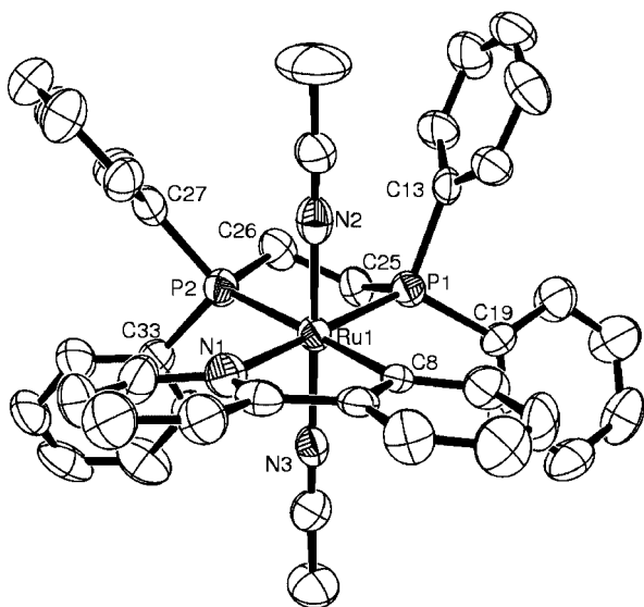
Figure 4. ORTEP view of the cationic part of compound 10 . Selected bond distances [Å] and angles [°]: Ru1–N3 2.001(6), Ru1–N2 2.001(6), Ru1–C8 2.096(6), Ru1–N1 2.118(5), Ru1–P1 2.343(2), Ru1–P2 2.373(2); N3–Ru1–N2 175.9(2), P1–Ru1–P2 83.08(6), C8–Ru1–N1 77.6(2), C8–Ru1–P1 100.42(17), N1–Ru1–P2 98.86(18).
